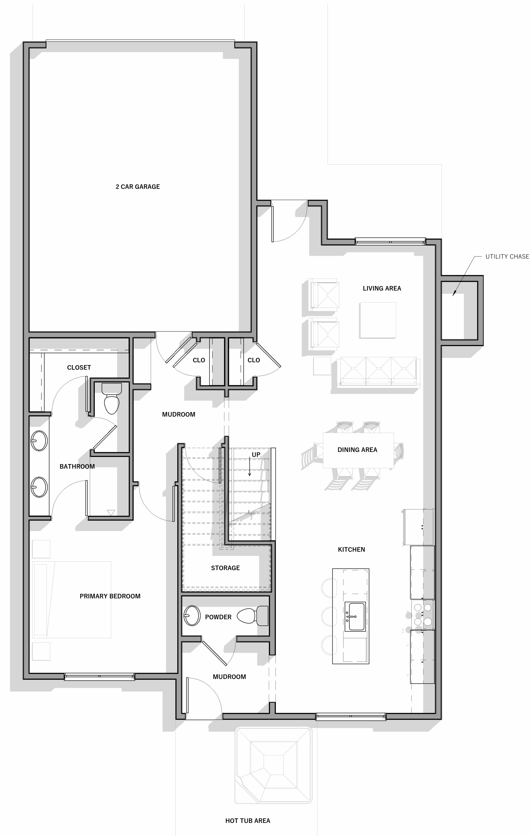
1 PR004 3 BEDROOM UNIT - LEVEL 1 1/4" = 1'-0"
